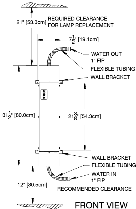
FRONT VIEW Figure 1A
